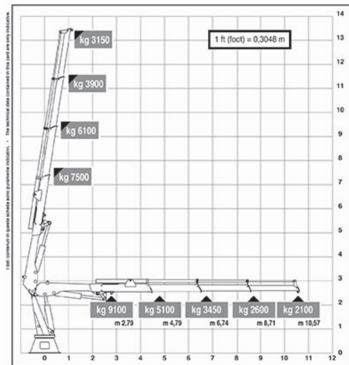
Jif Worker AFT Cranes HLRM 25-3S :
