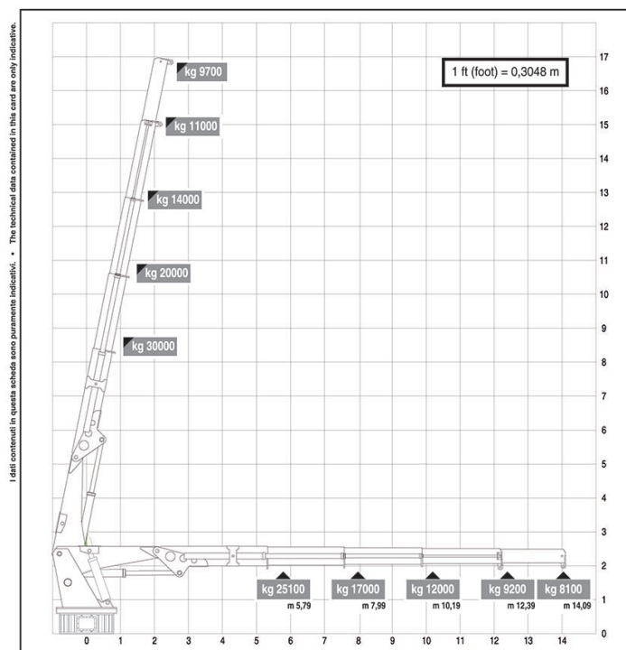
Jif Worker FWD Cranes HLRM 140-4S :
