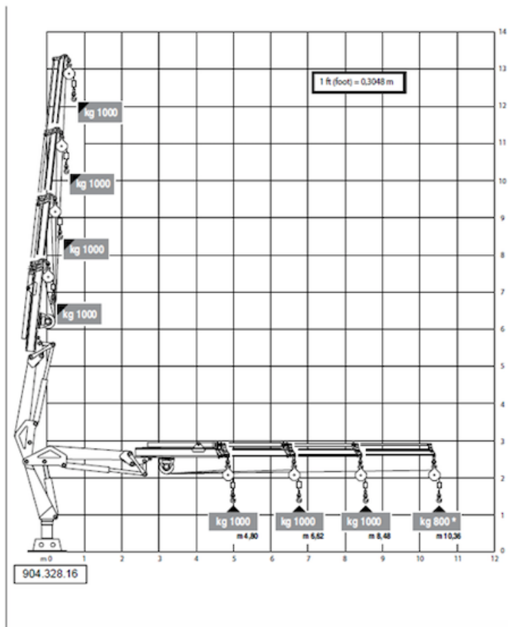
VDC TP Crane : with the use of the crane winch
