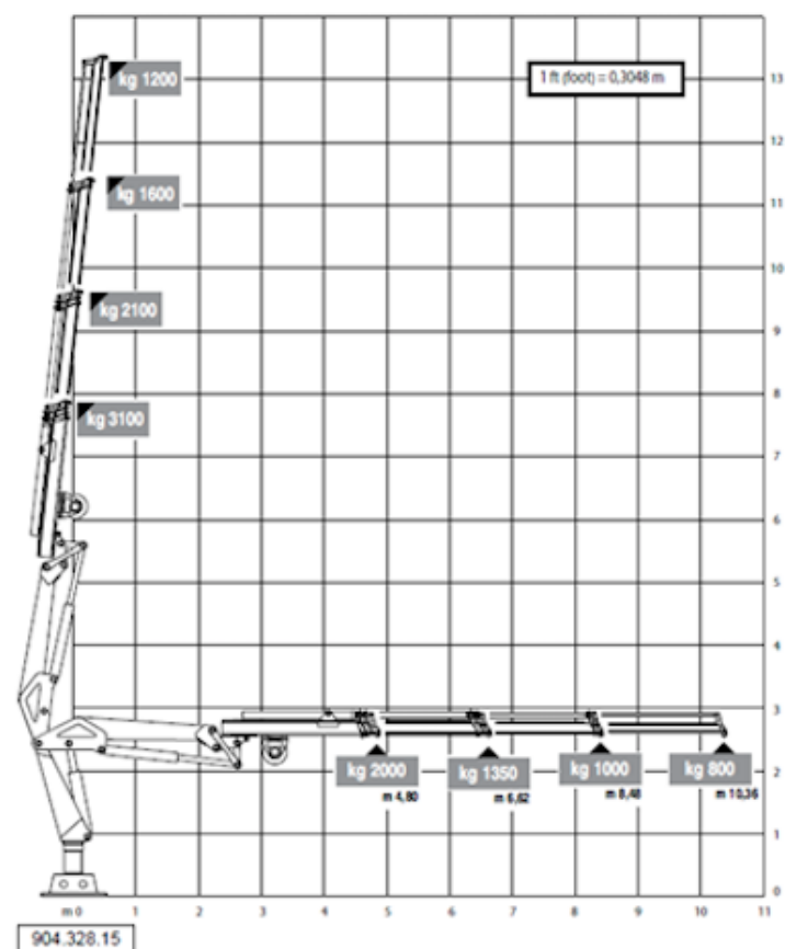
VDC TP Crane : without the use of the crane winch.
